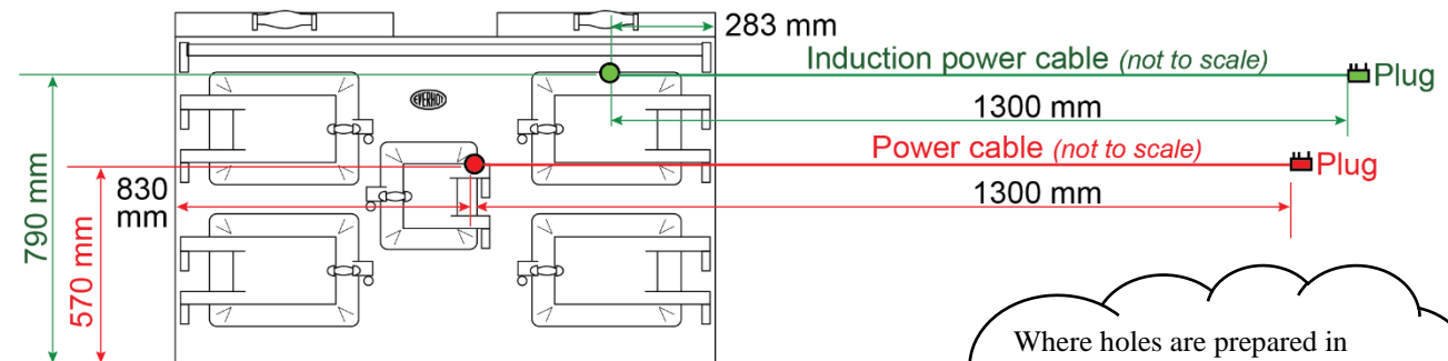
EVH 150i cable lengths
