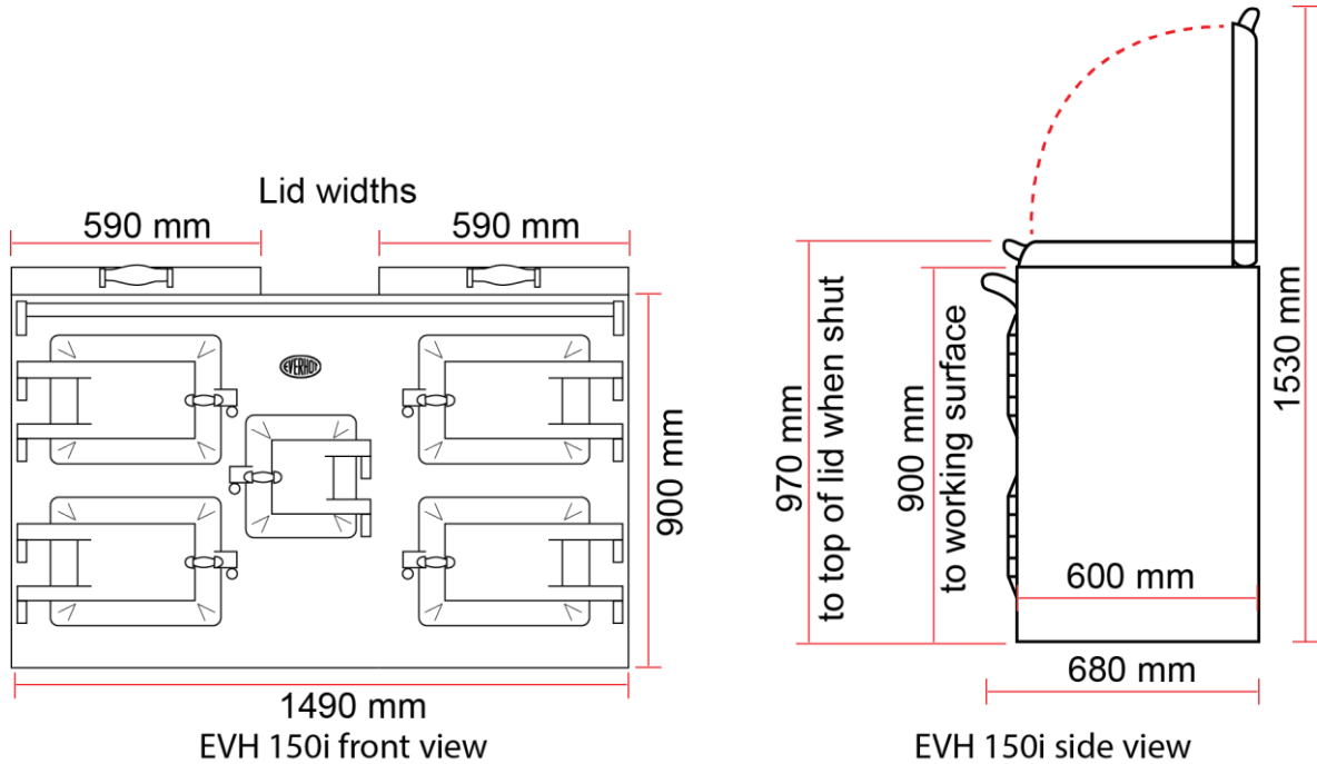
EVH150i dimensions
